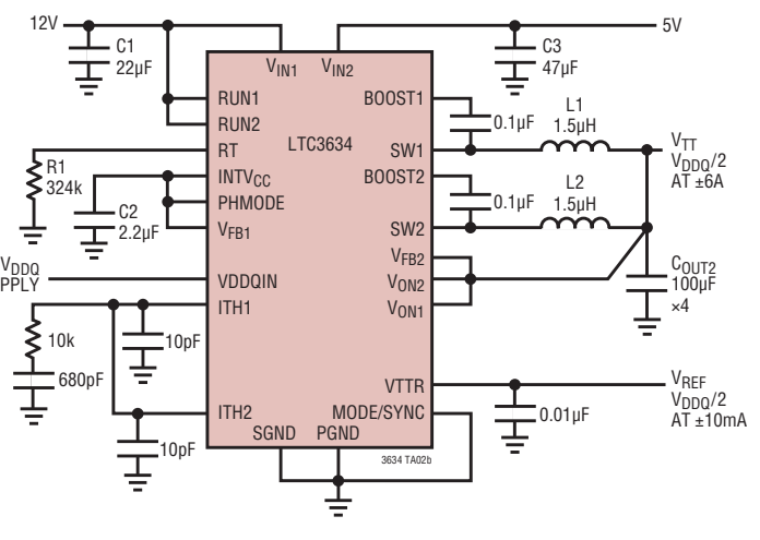
Figure 12b. 2-Phase V_{TT} Termination Using Two Input Supplies
