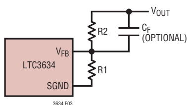
Figure 3. Setting the Output Voltage
