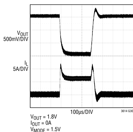
V_{OUT} Short to GND, Forced Continuous Mode
