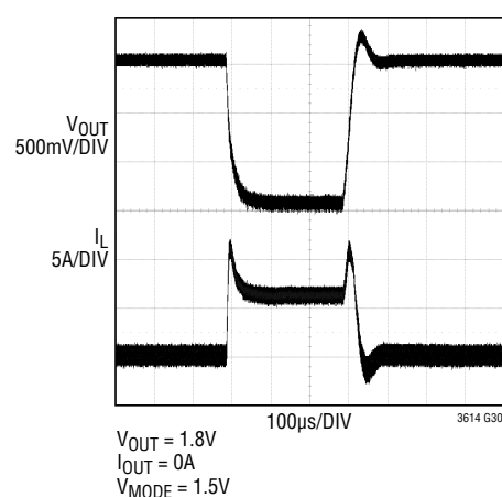
V_{OUT} Short to GND, Forced Continuous Mode
