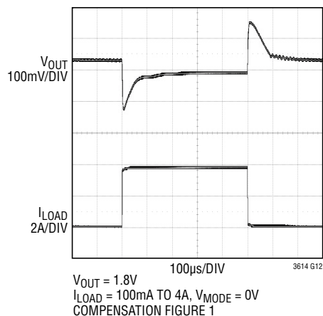
Load Step Transient in Forced Continuous Mode Sourcing and Sinking Current
