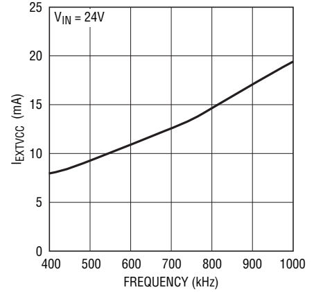
I EXTVCC vs Frequency
