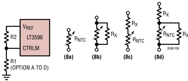
Figure 8. Programming the CTRL Pin
