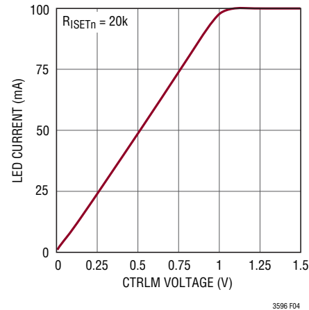
Figure 9. LED Current vs CTRL Voltage
