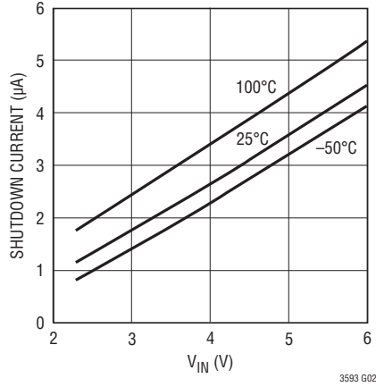
Shutdown Current ( V_{CTRL} = 0\text{V} )
