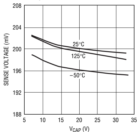
Sense Voltage ( V_{\text{CAP}} - V_{\text{LED}} ) vs V_{\text{CAP}}
