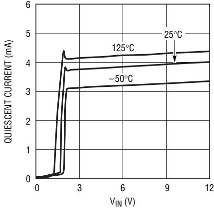
Quiescent Current ( V_{\text{CTRL}} = 3\text{V} )
