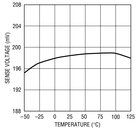
Sense Voltage ( V_{\text{CAP}} - V_{\text{LED}} ) vs Temperature
