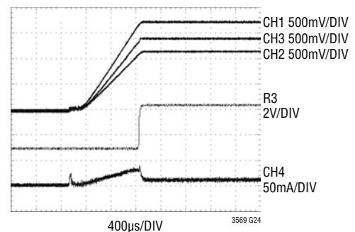
Soft-Start Into Light Load, PS, V_{IN} = 3.6\text{V} , CH1 = V_{OUT1} , CH2 = V_{OUT2} , CH3 = V_{OUT3} , CH4 = I_{IN} , R3 = PGOOD
