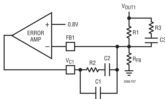
Figure 7. Error Amplifier with Type III Compensation
