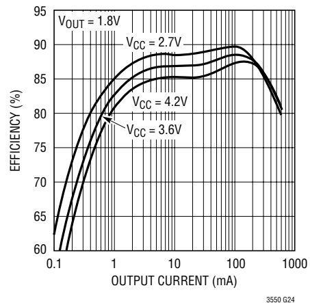
Figure 8b. Buck Regulator Efficiency vs Output Current
