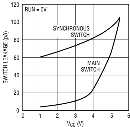
Switch Leakage Current vs V_{CC}
