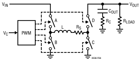
Figure 4. Small-Signal Model
