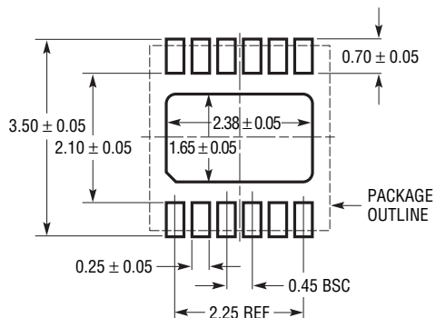
DC Package 12-Lead Plastic DFN (3mm × 3mm) (Reference LTC DWG # 05-08-1725 Rev A)
