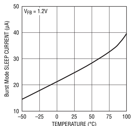
Burst Mode SLEEP Current vs Temperature
