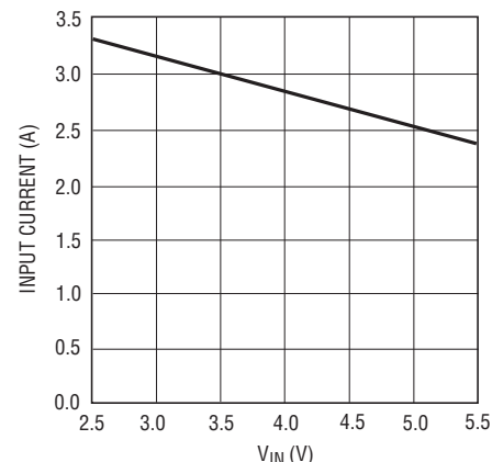
Peak Current Clamp vs V_{IN}
