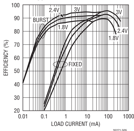
Efficiency vs Load Current and V_{IN} for V_{OUT2} = 3.3\text{V} at 1.2\text{MHz}
