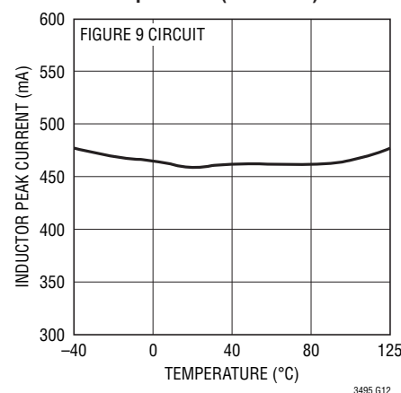
Peak Inductor Current vs Temperature (LT3495-1)
