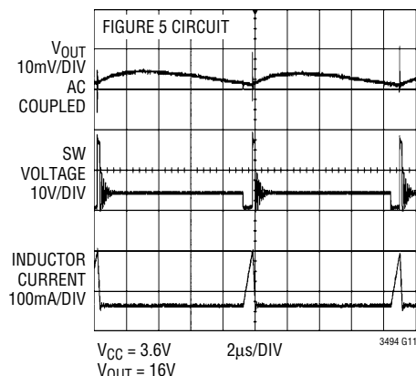
LT3494 Switching Waveforms at 1mA Load
