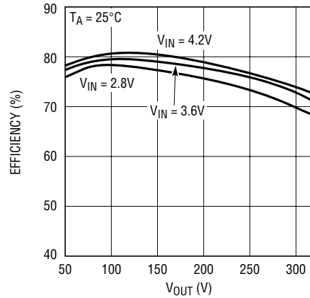
LT3468-1 Efficiency
