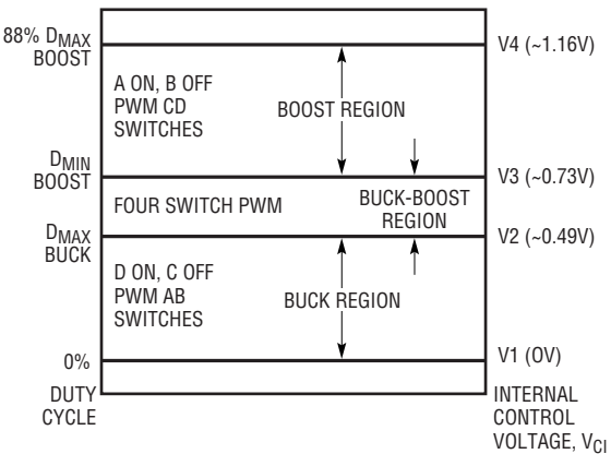
Figure 4. Switch Control vs Internal Control Voltage, V_{CI}
