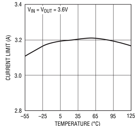
Current Limit
