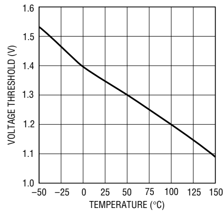
SYNC Pin Voltage Threshold vs Temperature
