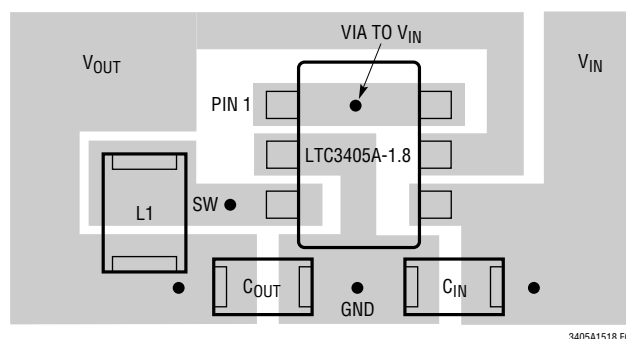
Figure 5. LTC3405A-1.8 Suggested Layout
