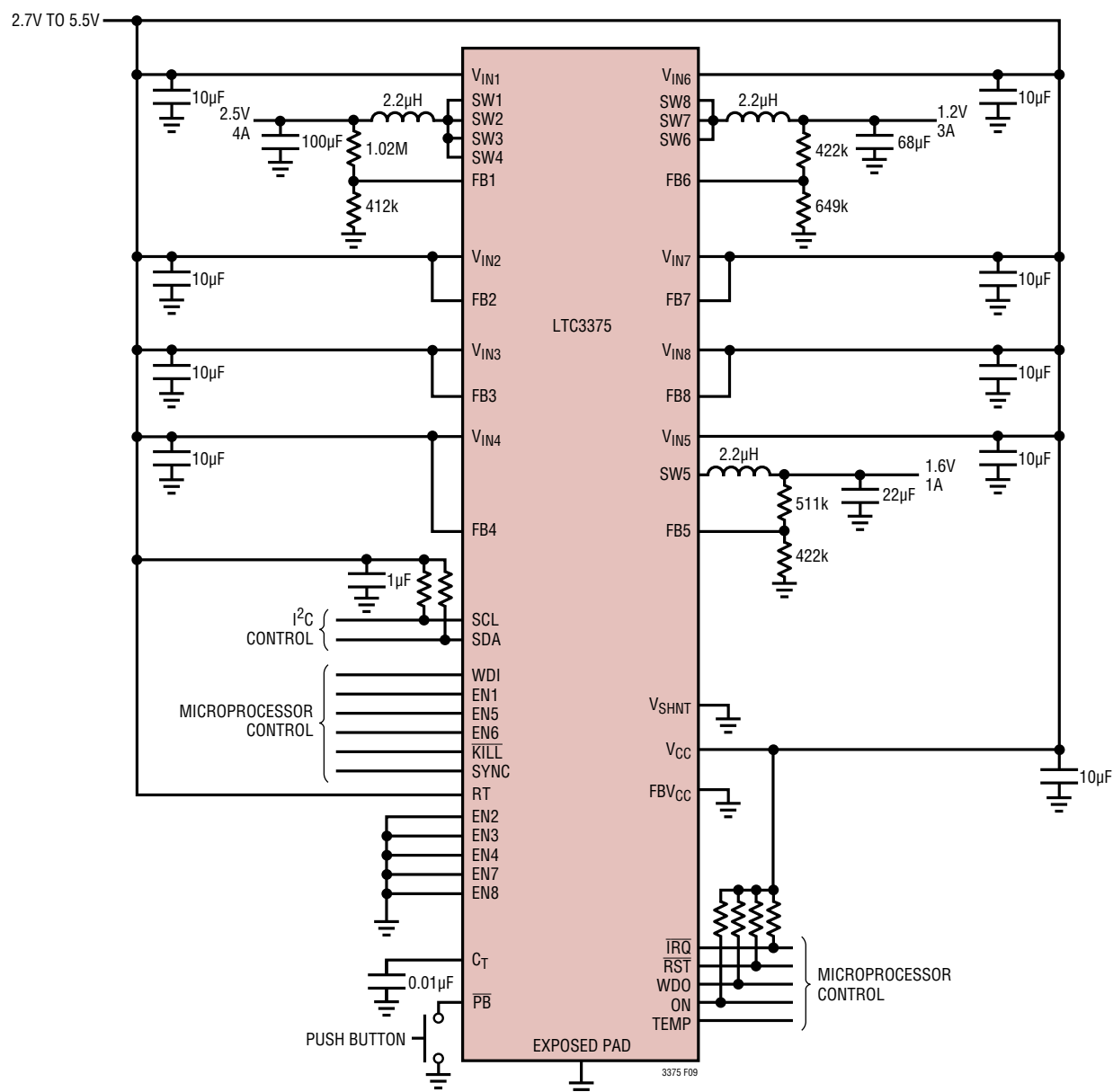
Figure 9. Combined Buck Regulators with Common Input Supply
