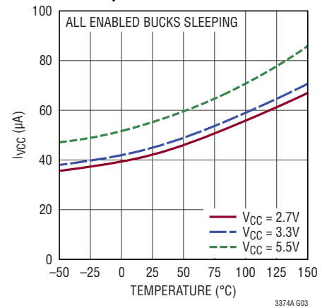
V_{CC} Quiescent Current vs Temperature
