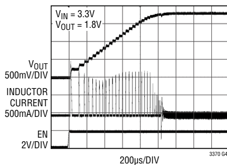
4A Buck Regulator No-Load Start-Up Transient (Forced Continuous Mode)
