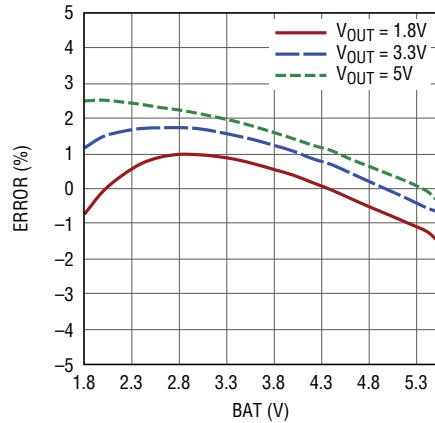
Total Unadjusted Coulomb Counter Error During Continuous Switching (150mA I_{PEAK} Setting)
