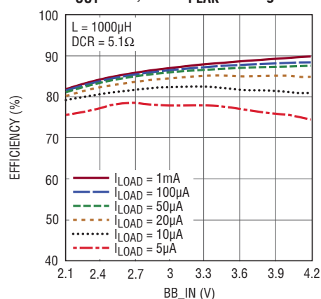
Buck-Boost Efficiency vs BB_IN for V_{OUT} = 5\text{V} , 5mA I_{PEAK} Setting
