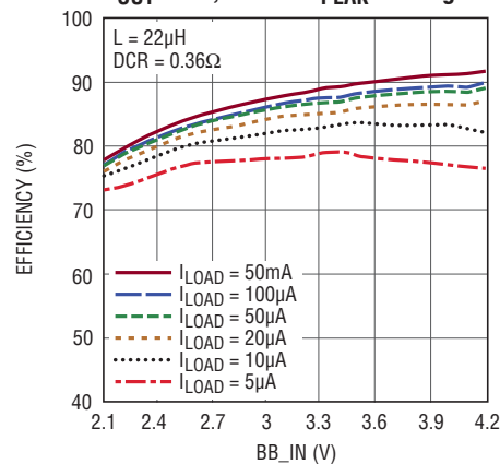
Buck-Boost Efficiency vs BB_IN for V_{OUT} = 5\text{V} , 250mA I_{PEAK} Setting
