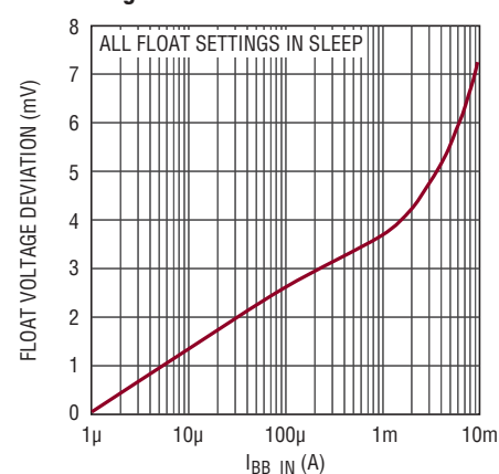
Shunt Float Voltage Load Regulation
