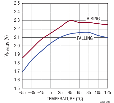
V REG,UV vs Temperature
