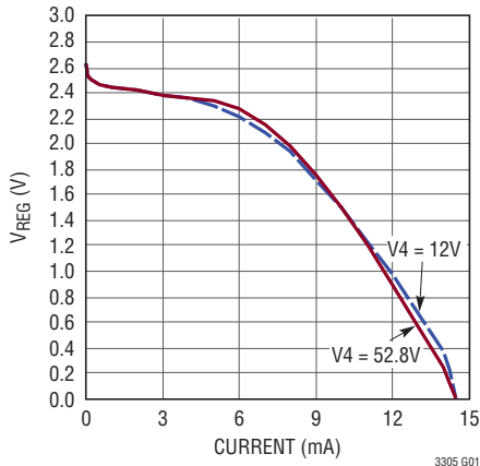
V REG Line and Load Regulation
