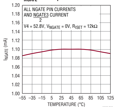
I NGATE vs Temperature
