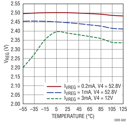
V REG vs Temperature
