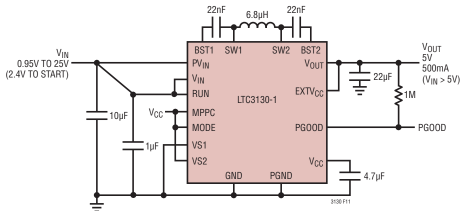
Figure 11. Low Noise, Wide V_{IN} Range 5V Converter
