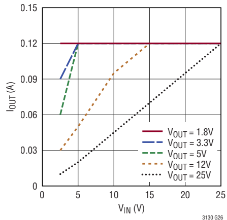
Burst Mode Operation, Load Current Threshold vs V_{IN} and V_{OUT} (MODE = 0V)
