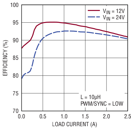
Efficiency, V_{OUT} = 5V , f_{SW} = 700\text{kHz}
