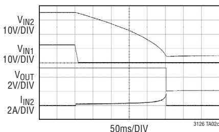
V_{OUT} Hold-Up with Loss of Input Supply
