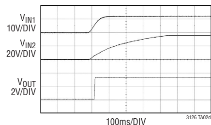
Power-Up Waveforms
