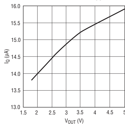
Burst Mode Current vs V_{OUT}
