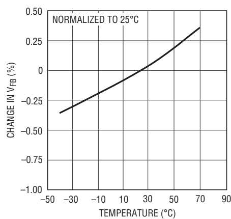
Current Sense Voltage ( V_{RPROG} ) vs Temperature
