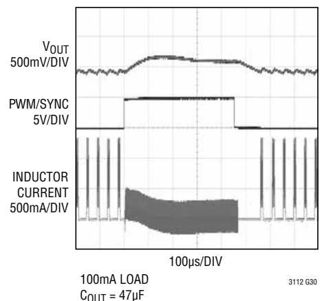
5V_{IN} to 5.0V_{OUT} Burst to PWM Waveforms,
