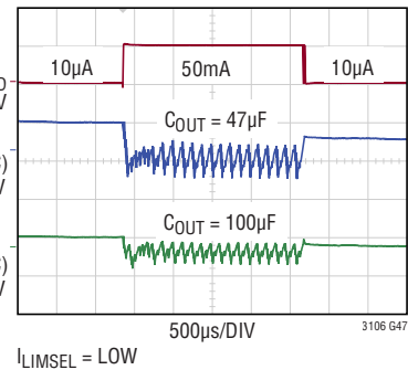
5V V_{IN} to 1.8V V_{OUT} Load Step 10 \mu A to 50mA
