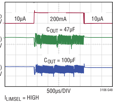
5V V_{IN} to 1.8V V_{OUT} Load Step 10 \mu A to 200mA
