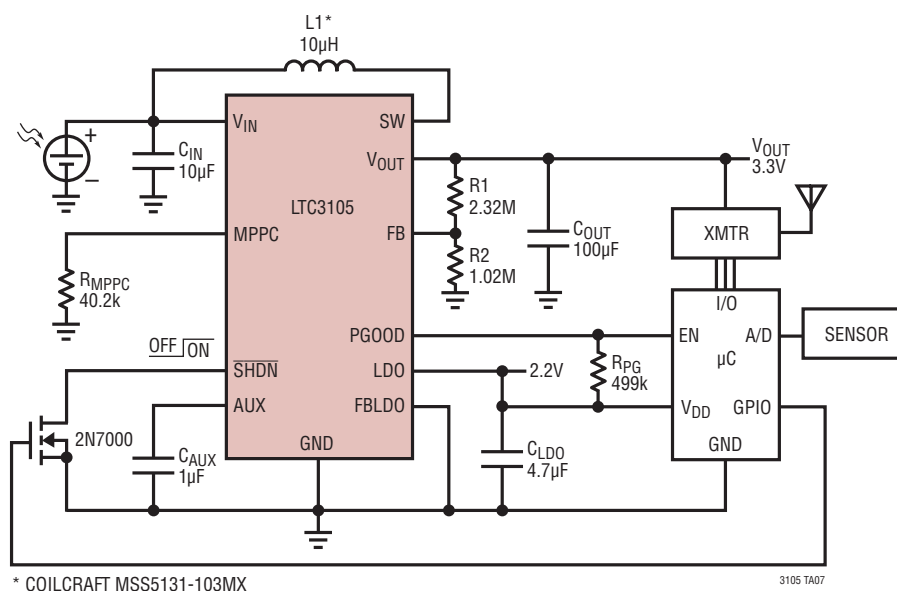
Single-Cell Powered Remote Wireless Sensor
