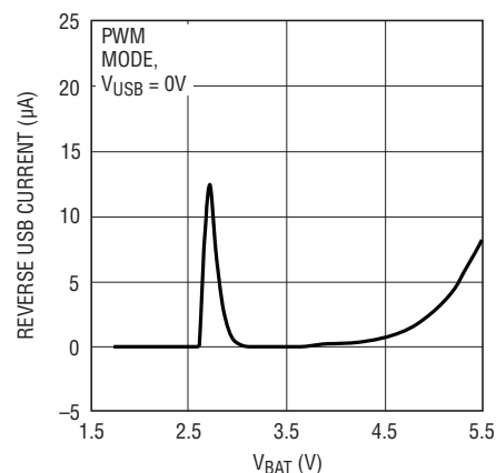
Reverse USB Current vs BAT Voltage
