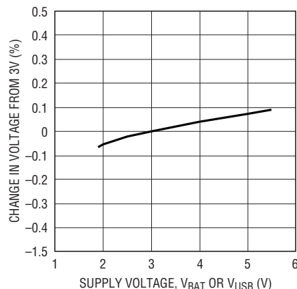
LDO Output Voltage vs Supply Voltage
