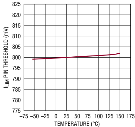
I_{LIM} Pin Threshold Voltage
