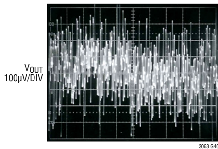
5V 10Hz to 100kHz Output Noise C_{\text{REF/BYP}} = 10\text{nF} , C_{\text{FF}} = 0
