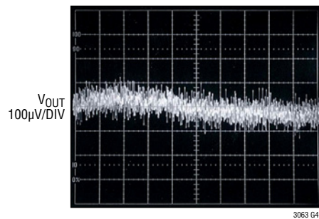
5V 10Hz to 100kHz Output Noise C_{\text{REF/BYP}} = 10\text{nF} , C_{\text{FF}} = 10\text{nF}
