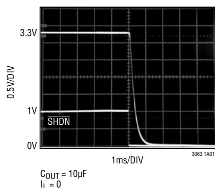
LT3063-3.3 Active Output Discharge
