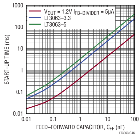
Start-Up Time vs CFF
