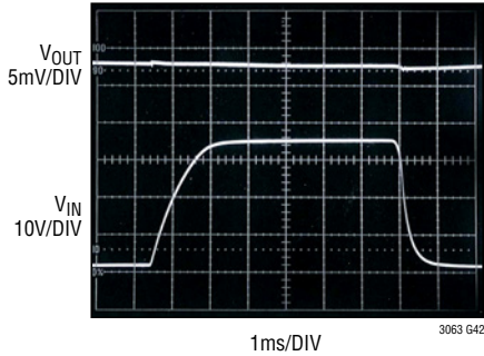
Transient Response, V_{OUT} = 5V Load Dump, V_{IN} = 12V to 45V
