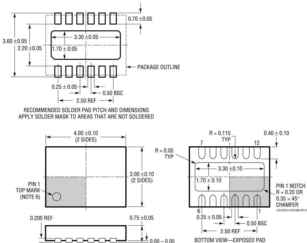
DE/UE Package 12-Lead Plastic DFN (4mm × 3mm) (Reference LTC DWG # 05-08-1695 Rev D)
