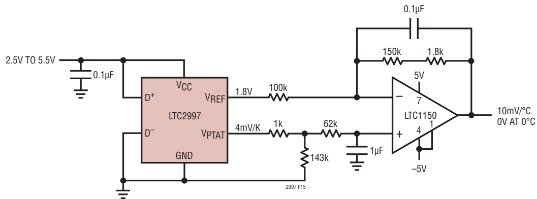
Figure 15. Celsius Thermometer
