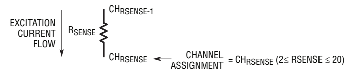
Figure 8. Sense Resistor Channel Assignment Convention for 2-Wire RTDs
