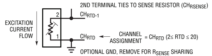
Figure 7. 2-Wire RTD Channel Assignment Convention
