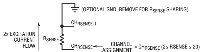
Sense resistor channel assignments follow the general convention shown in Figure 11. The sense resistor is tied between CH_{RSENSE} and CH_{RSENSE-1} , where CH_{RSENSE} is tied to the 3rd terminal of the RTD and CH_{RSENSE-1} is tied to ground (or left floating for R_{SENSE} sharing). Channel assignment data (see Table 33) is mapped into the memory location corresponding to CH_{RSENSE} .
