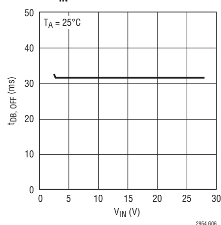
Turn-Off Debounce Time ( t_{\text{DB,OFF}} ) vs V_{\text{IN}}
