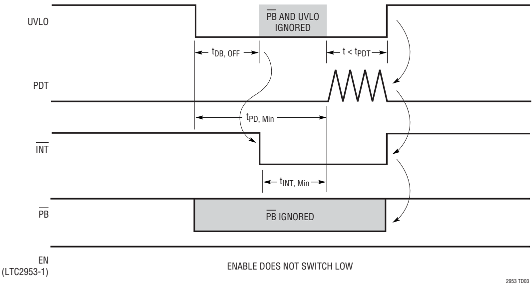
Figure 3. UVLO Interrupt Pulse: \overline{\text{UVLO}} Low for t_{\text{DB, OFF}} < t < (t_{\text{PD, Min}} + t_{\text{PDT}}) (Enable Remains Active)
