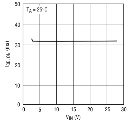
Turn On Debounce Time ( t_{DB, ON} ) vs V_{IN}
