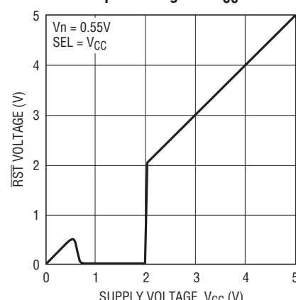
\overline{RST} Output Voltage vs V_{CC}
