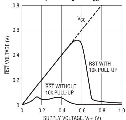
\overline{RST} Output Voltage vs V_{CC}
