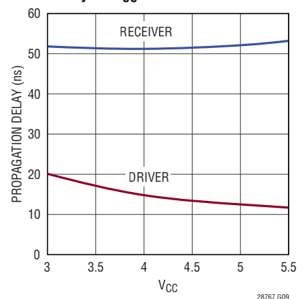
Driver and Receiver Propagation Delay vs V_{CC}
