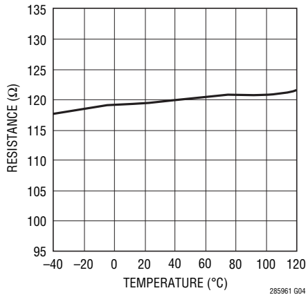
R_{\text{TERM}} vs Temperature
